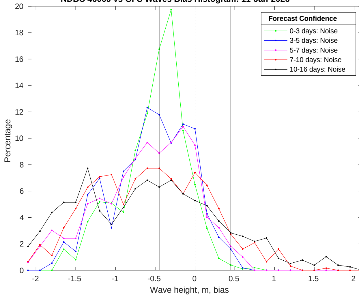
NDBC 46069 vs GFS Waves Bias Histogram: 11-Jan-2026
