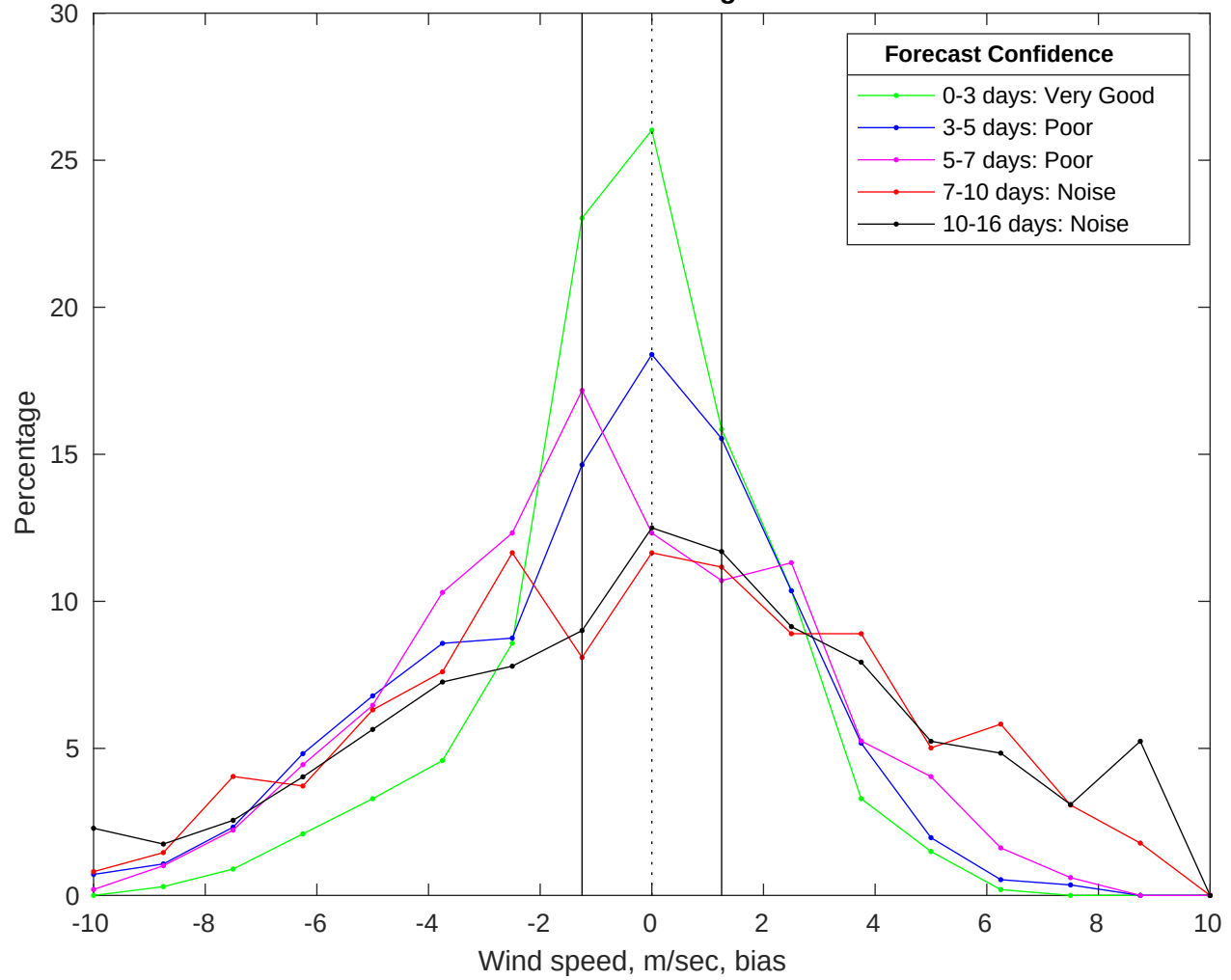
NDBC 46069 vs GFS Winds Bias Histogram: 11-Jan-2026
