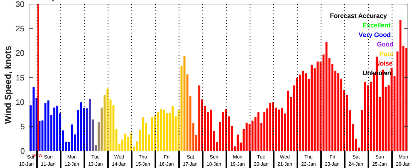
GFS Wind Speed Forecast for NDBC 46069 from 10-Jan-2026 16:00:00 to 26-Jan-2026 16:00:00
