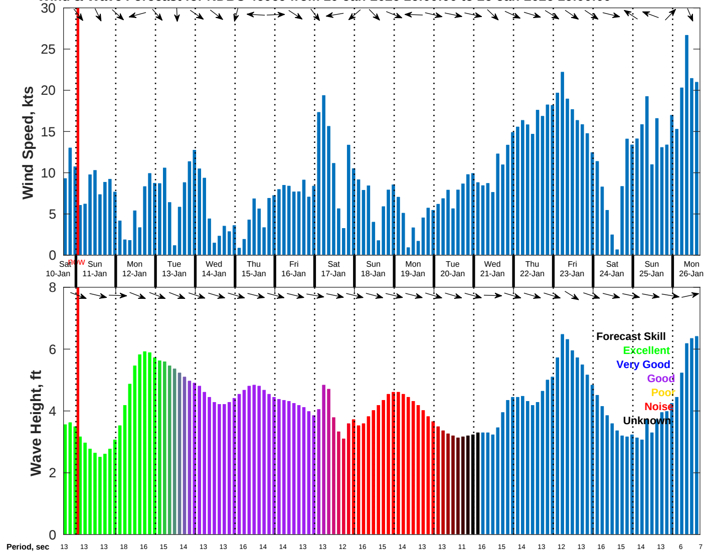
Wind & Wave Forecast for NDBC 46069 from 10-Jan-2026 16:00:00 to 26-Jan-2026 16:00:00
