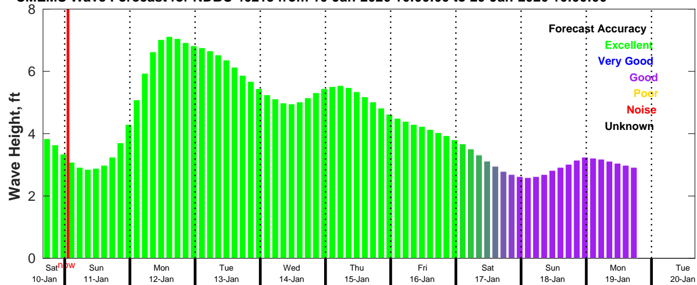
CMEMS Wave Forecast for NDBC 46215 from 10-Jan-2026 16:00:00 to 20-Jan-2026 16:00:00
