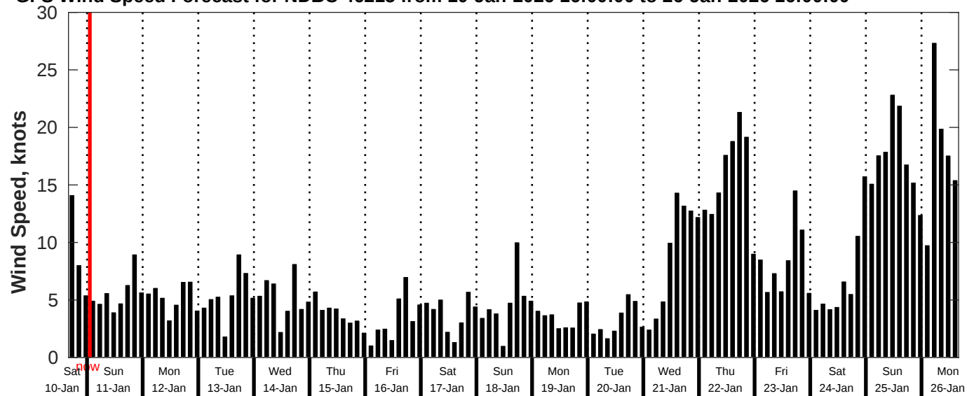
GFS Wind Speed Forecast for NDBC 46215 from 10-Jan-2026 16:00:00 to 26-Jan-2026 16:00:00
