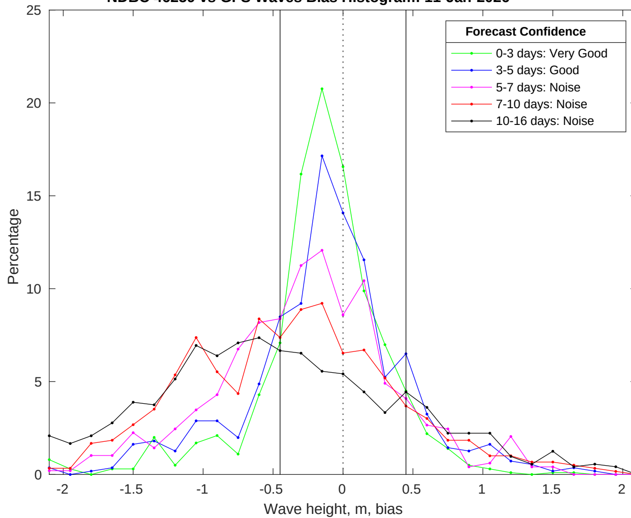
NDBC 46259 vs GFS Waves Bias Histogram: 11-Jan-2026
