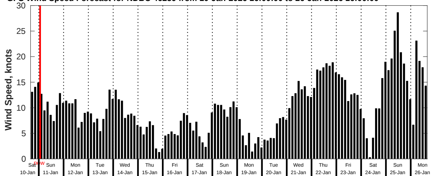
GFS Wind Speed Forecast for NDBC 46259 from 10-Jan-2026 16:00:00 to 26-Jan-2026 16:00:00
