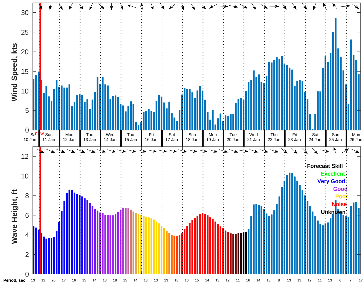
Wind & Wave Forecast for NDBC 46259 from 10-Jan-2026 16:00:00 to 26-Jan-2026 16:00:00
