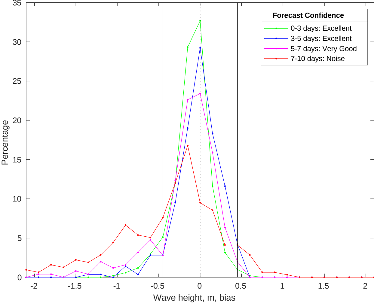
NDBC 51000 vs CMEMS Waves Bias Histogram: 11-Jan-2026
