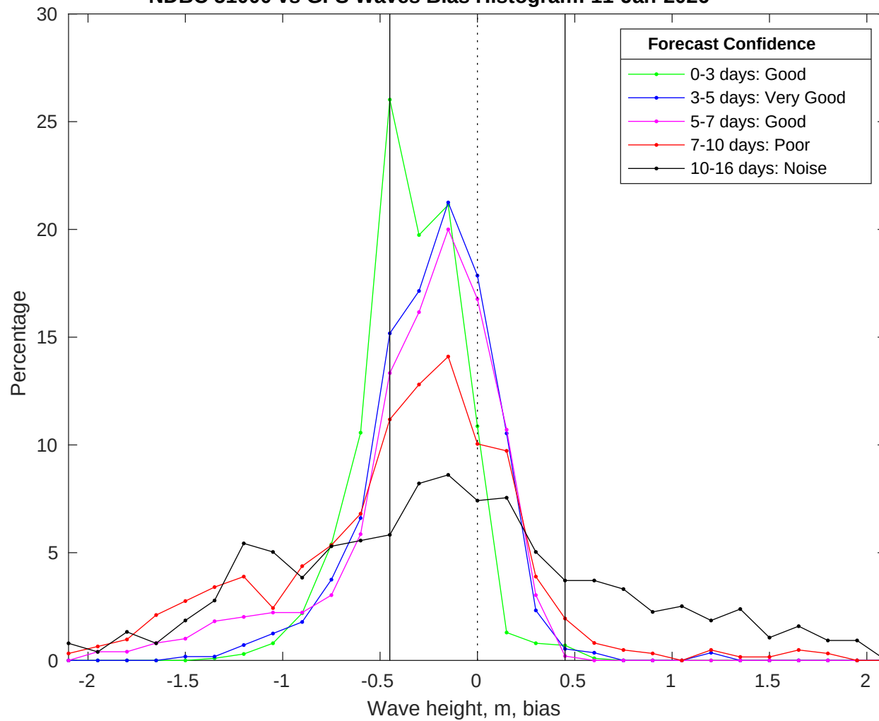
NDBC 51000 vs GFS Waves Bias Histogram: 11-Jan-2026
