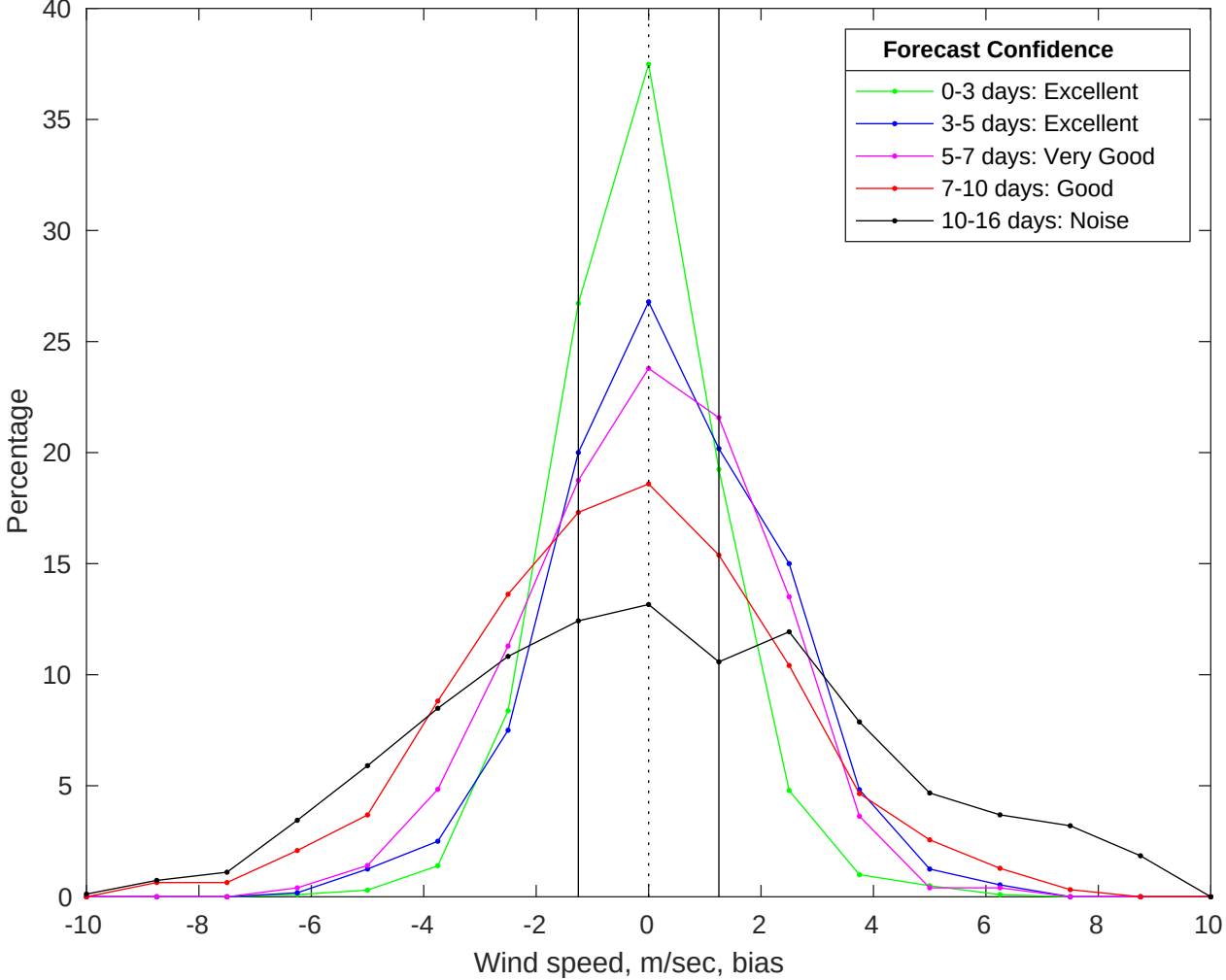
NDBC 51000 vs GFS Winds Bias Histogram: 11-Jan-2026
