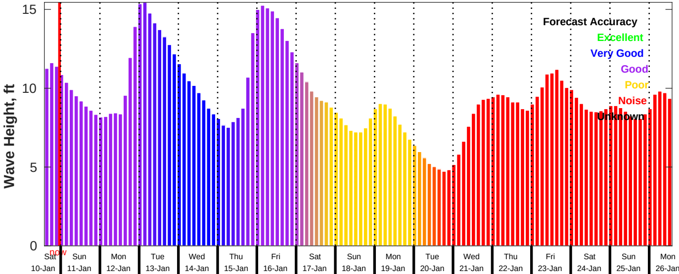
GFS Wave Forecast for NDBC 51000 from 10-Jan-2026 14:00:00 to 26-Jan-2026 14:00:00
