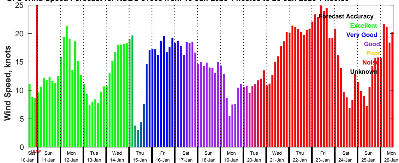
GFS Wind Speed Forecast for NDBC 51000 from 10-Jan-2026 14:00:00 to 26-Jan-2026 14:00:00
