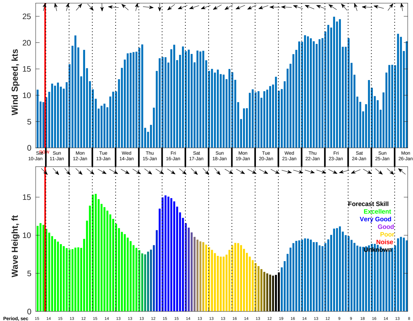
Wind & Wave Forecast for NDBC 51000 from 10-Jan-2026 14:00:00 to 26-Jan-2026 14:00:00
