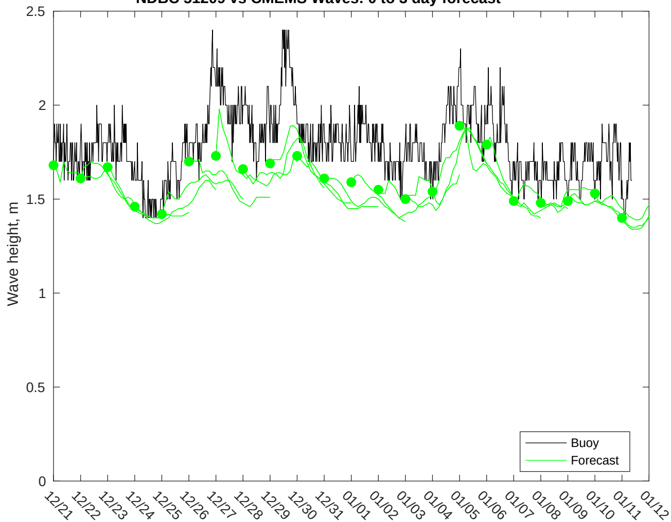
NDBC 51209 vs CMEMS Waves: 0 to 3 day forecast
