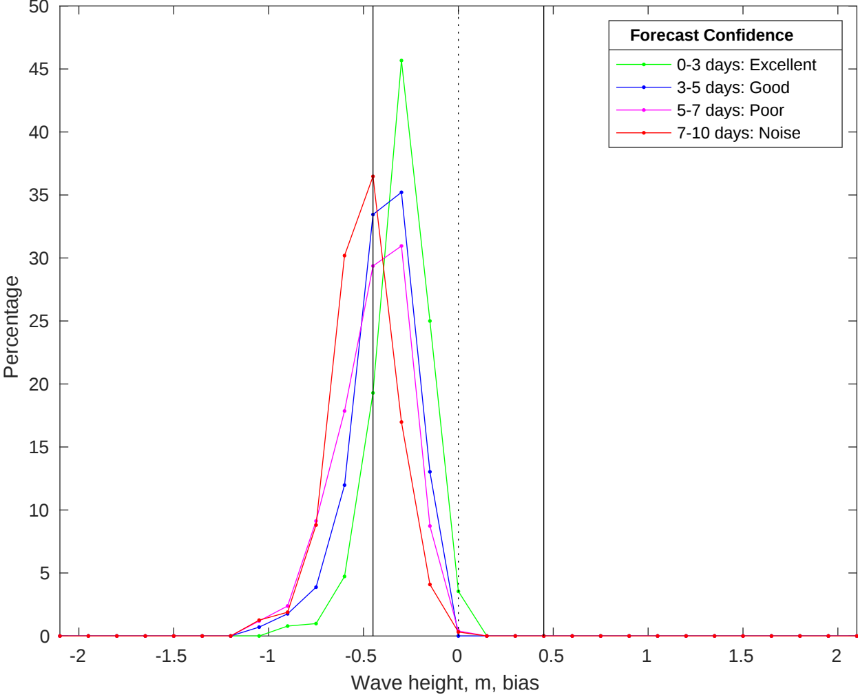
NDBC 51209 vs CMEMS Waves Bias Histogram: 11-Jan-2026
