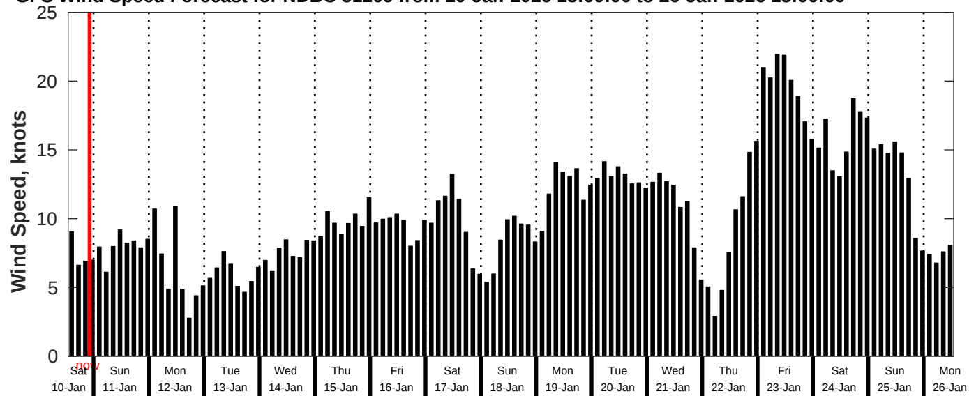
GFS Wind Speed Forecast for NDBC 51209 from 10-Jan-2026 13:00:00 to 26-Jan-2026 13:00:00
