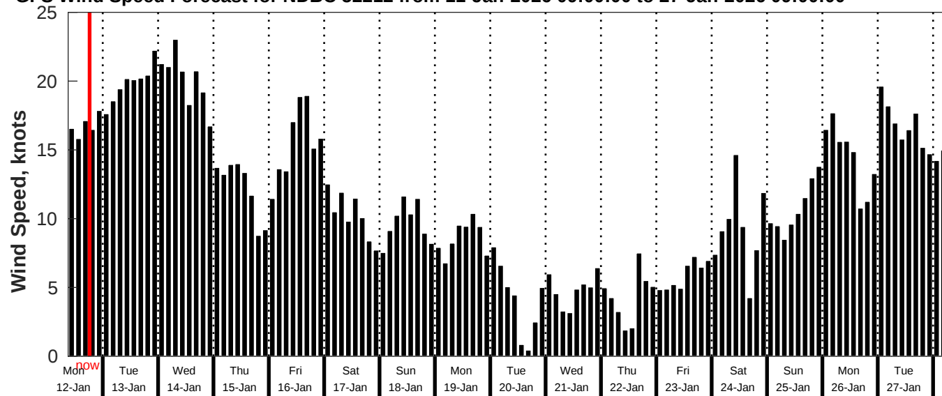
GFS Wind Speed Forecast for NDBC 52212 from 11-Jan-2026 09:00:00 to 27-Jan-2026 09:00:00
