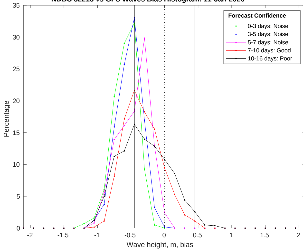
NDBC 52213 vs GFS Waves Bias Histogram: 11-Jan-2026
