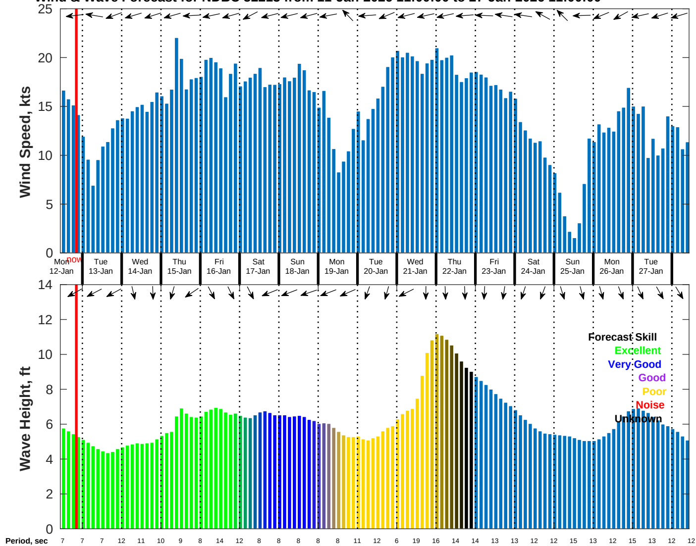
Wind & Wave Forecast for NDBC 52213 from 11-Jan-2026 11:00:00 to 27-Jan-2026 11:00:00
