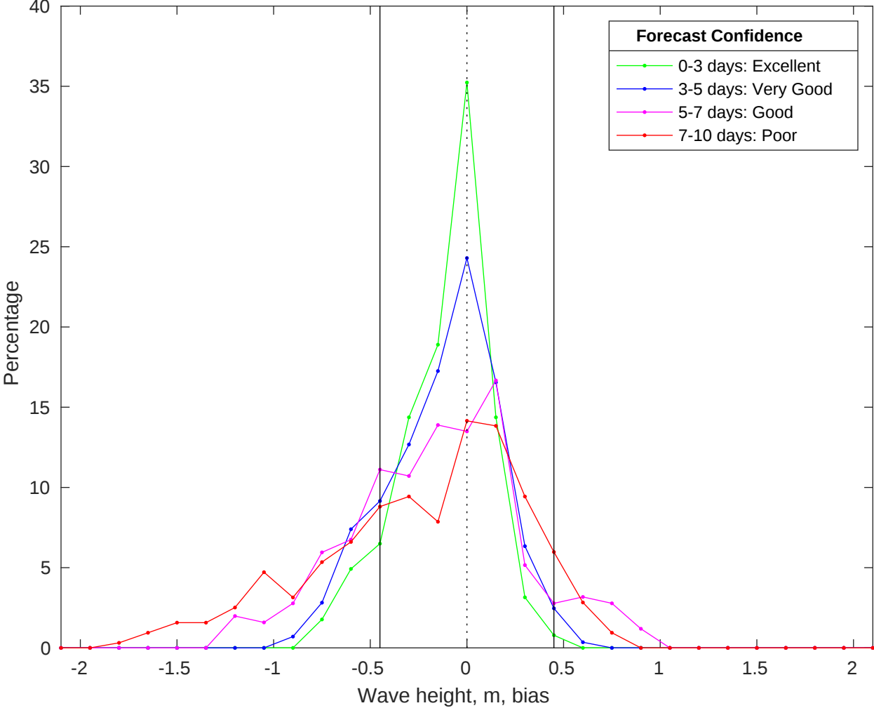
NDBC 41004 vs CMEMS Waves Bias Histogram: 12-Jan-2026
