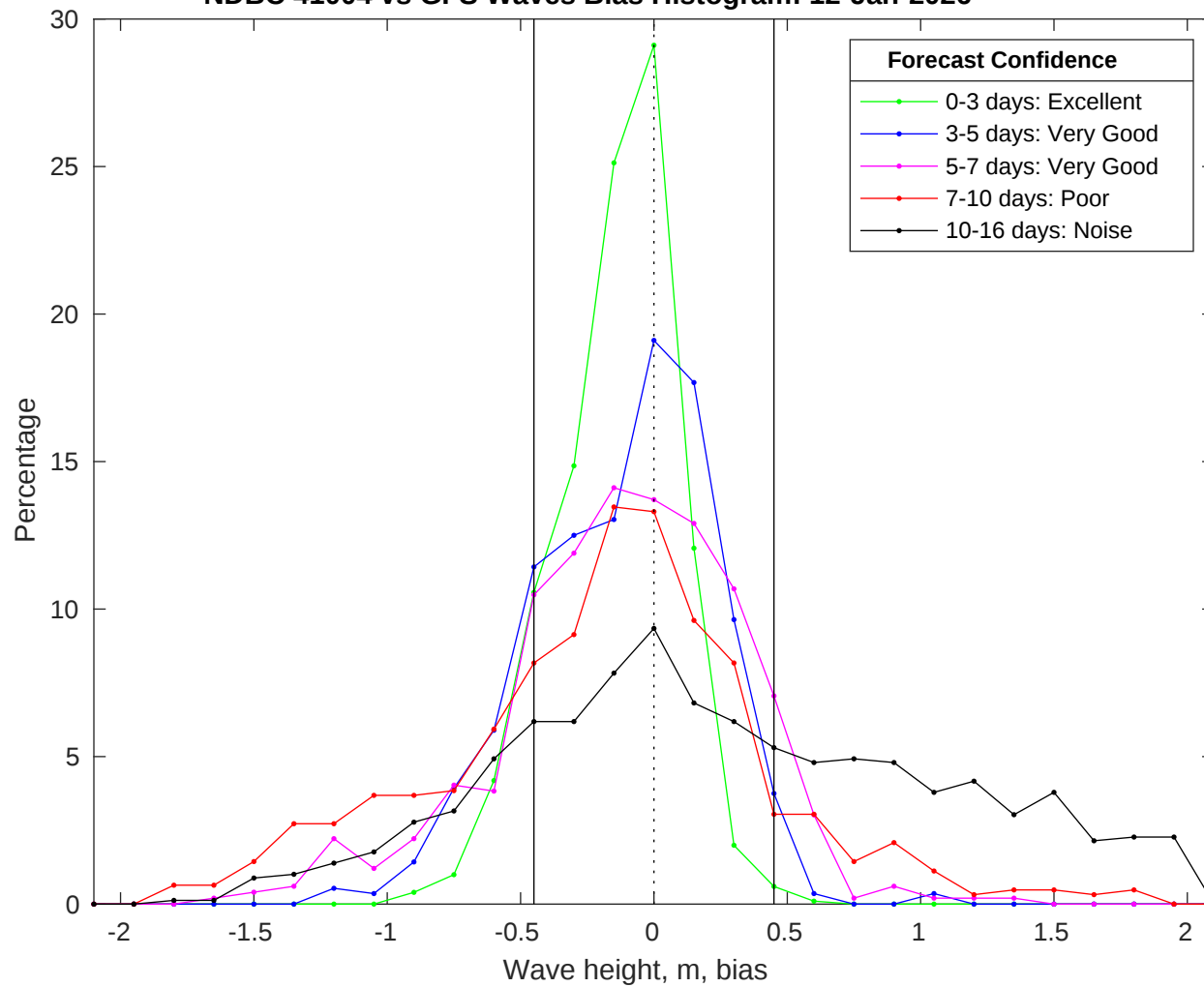
NDBC 41004 vs GFS Waves Bias Histogram: 12-Jan-2026
