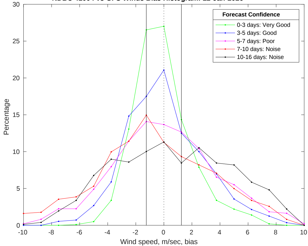
NDBC 41004 vs GFS Winds Bias Histogram: 12-Jan-2026
