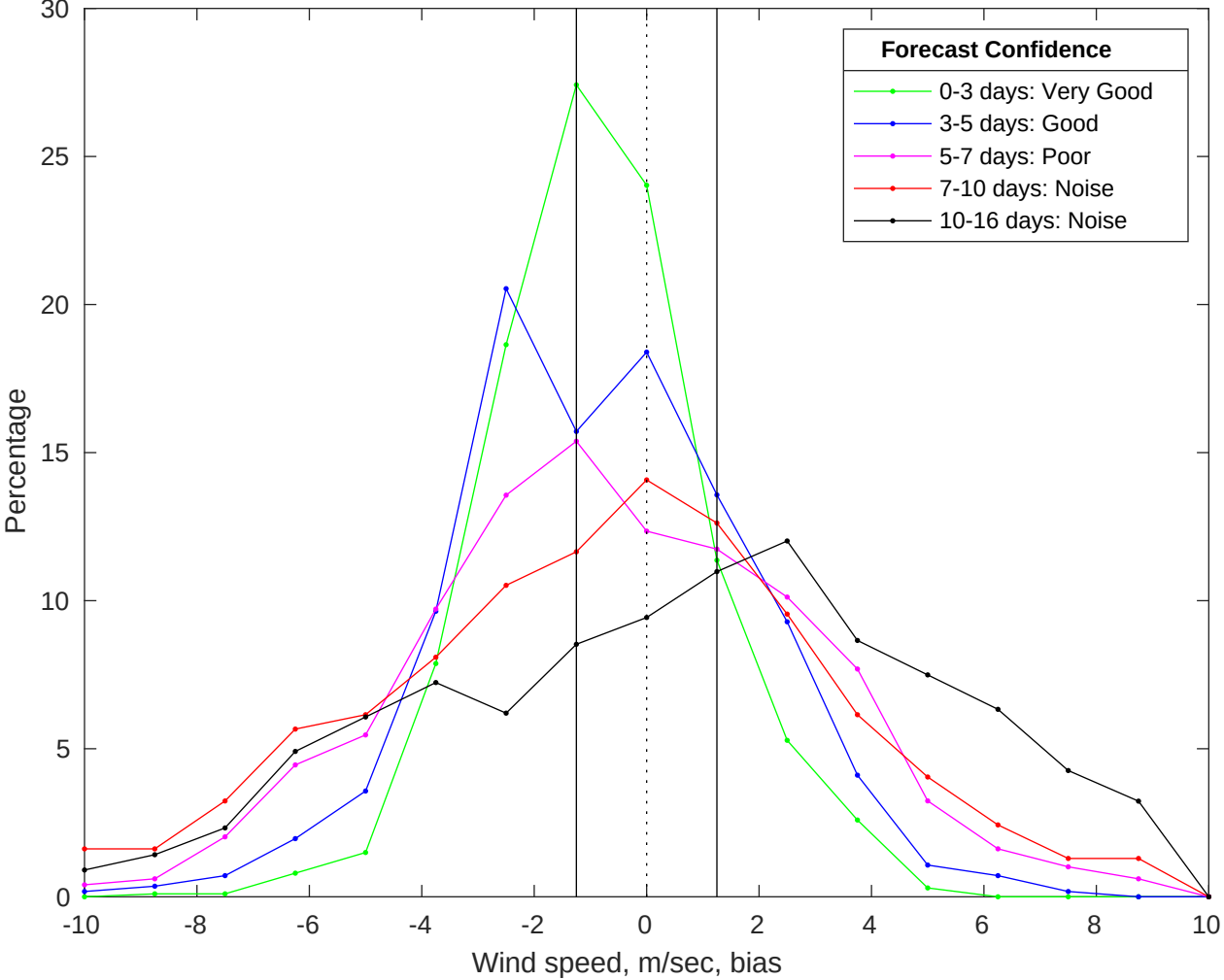
NDBC 41013 vs GFS Winds Bias Histogram: 12-Jan-2026
