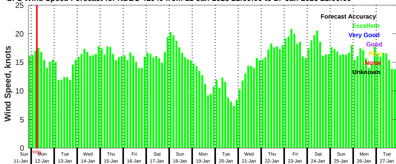
GFS Wind Speed Forecast for NDBC 41040 from 11-Jan-2026 21:00:00 to 27-Jan-2026 21:00:00
