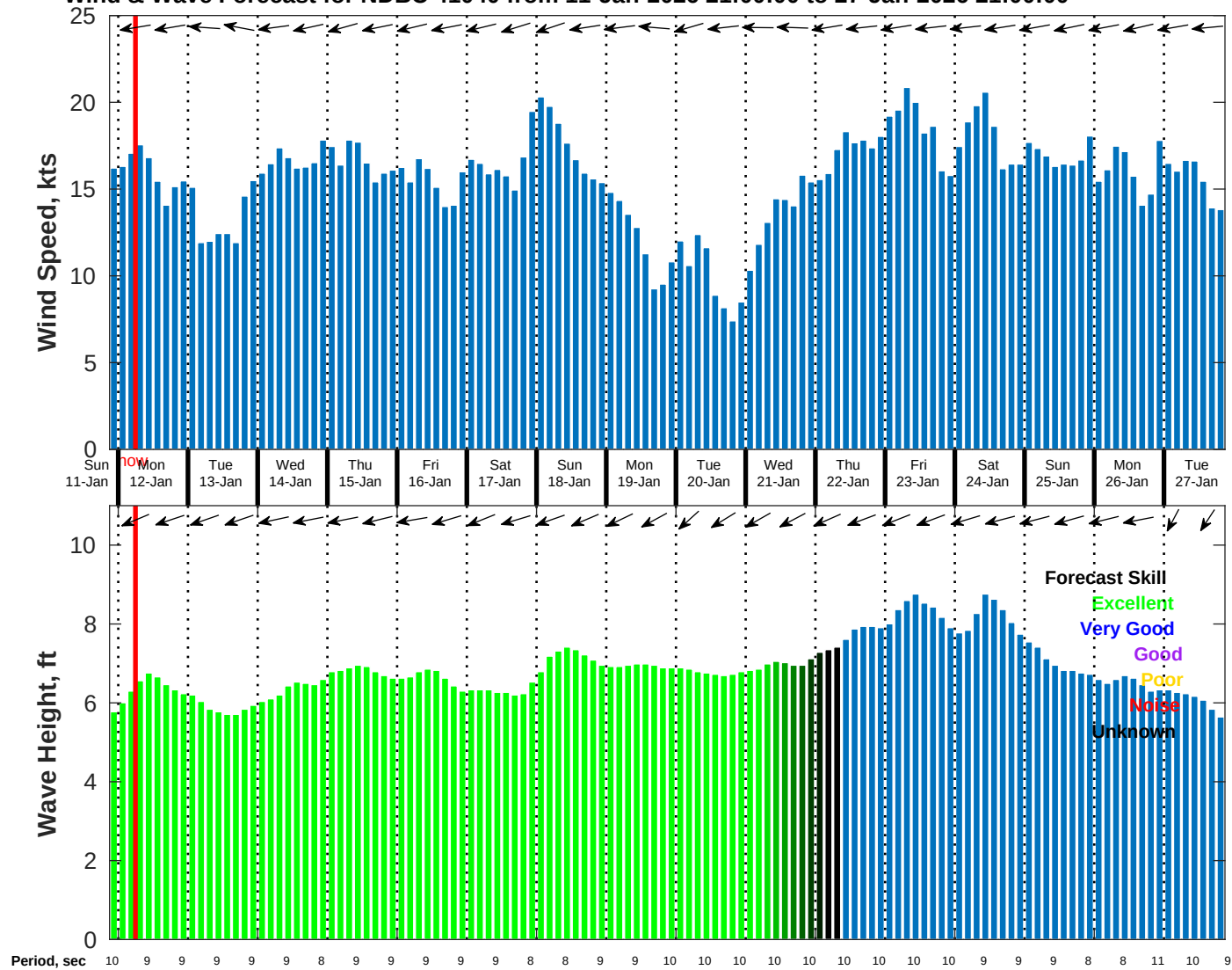
Wind & Wave Forecast for NDBC 41040 from 11-Jan-2026 21:00:00 to 27-Jan-2026 21:00:00
