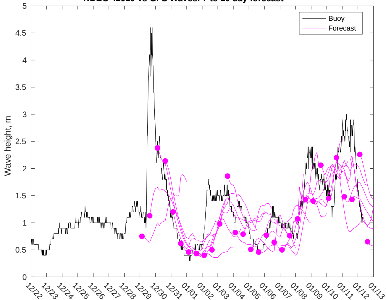
NDBC 42019 vs GFS Waves: 7 to 10 day forecast
