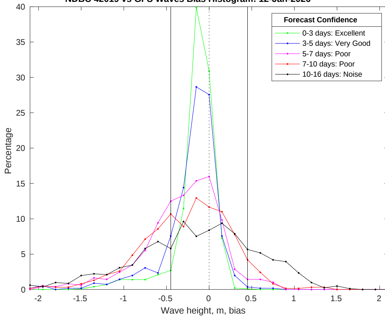
NDBC 42019 vs GFS Waves Bias Histogram: 12-Jan-2026
