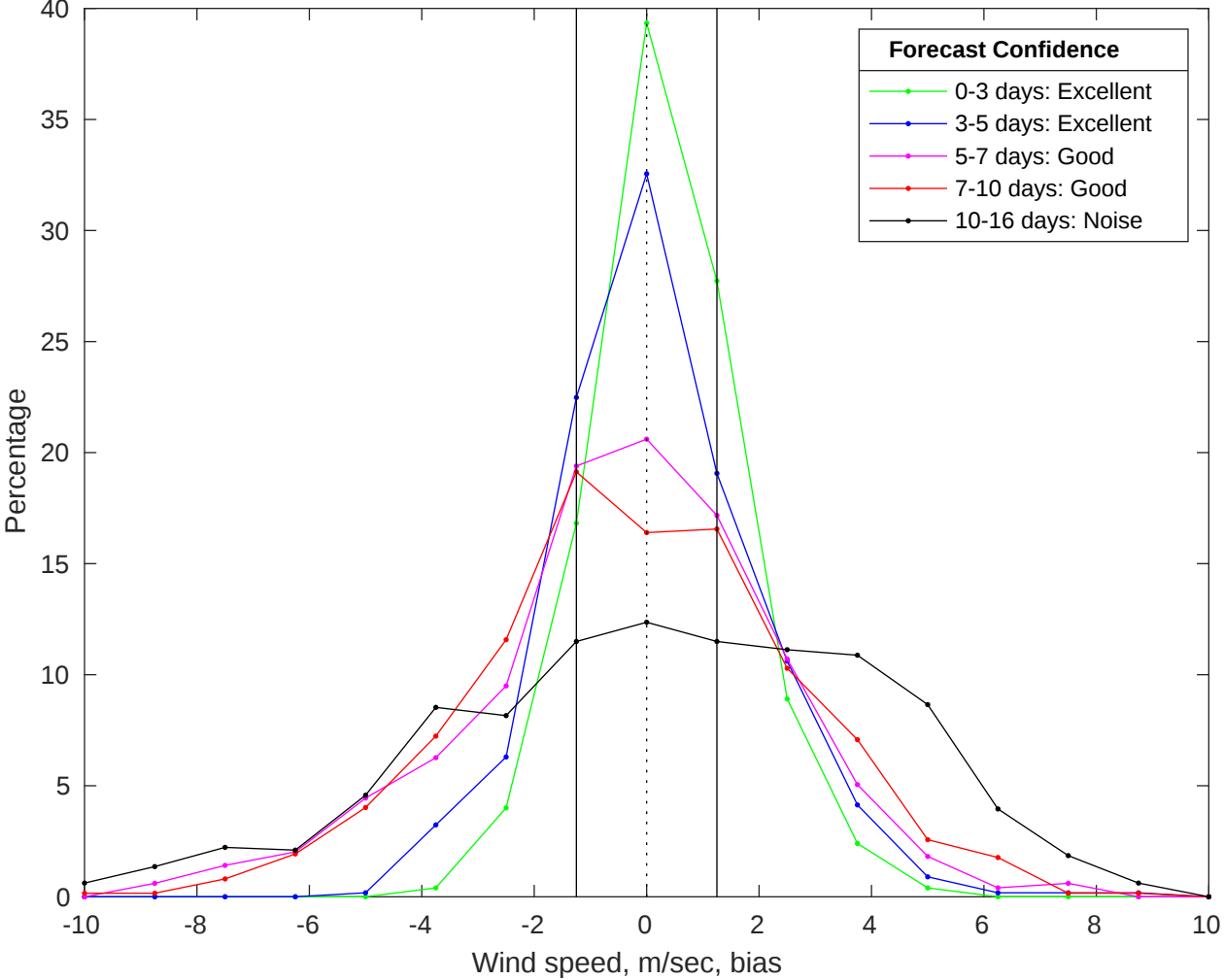
NDBC 42019 vs GFS Winds Bias Histogram: 12-Jan-2026
