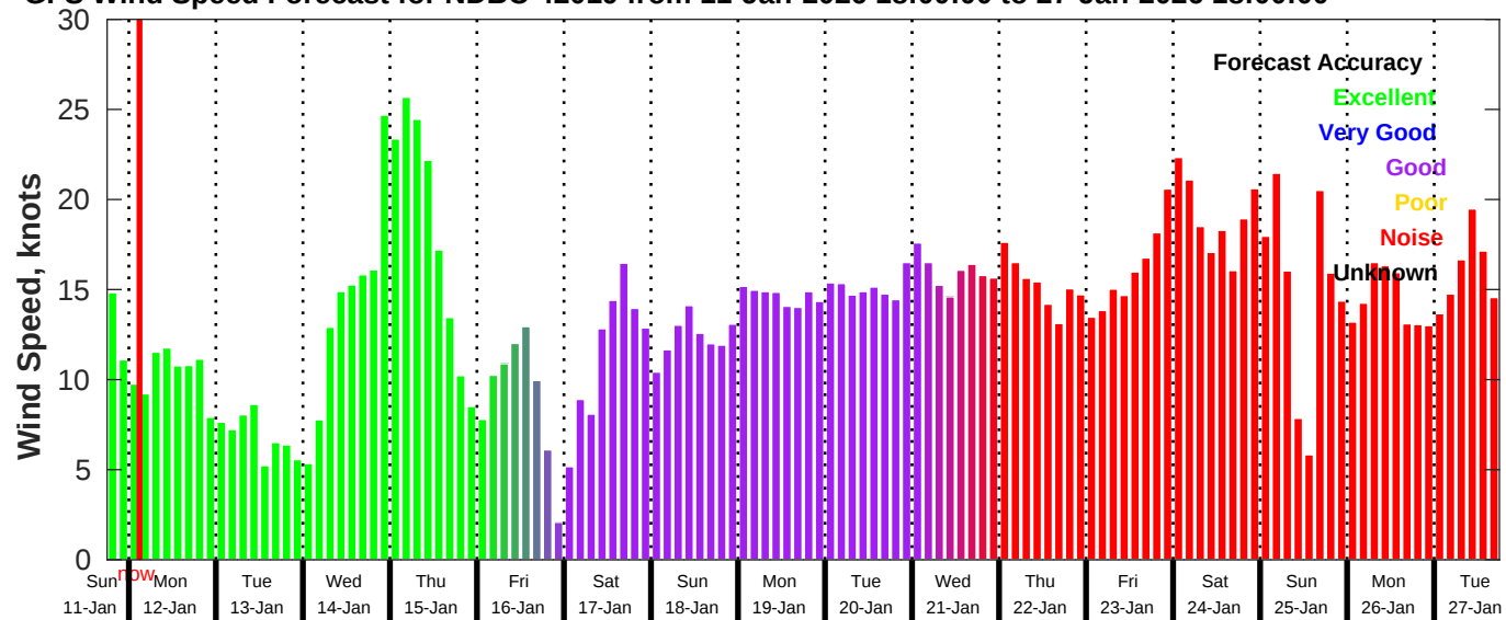
GFS Wind Speed Forecast for NDBC 42019 from 11-Jan-2026 18:00:00 to 27-Jan-2026 18:00:00
