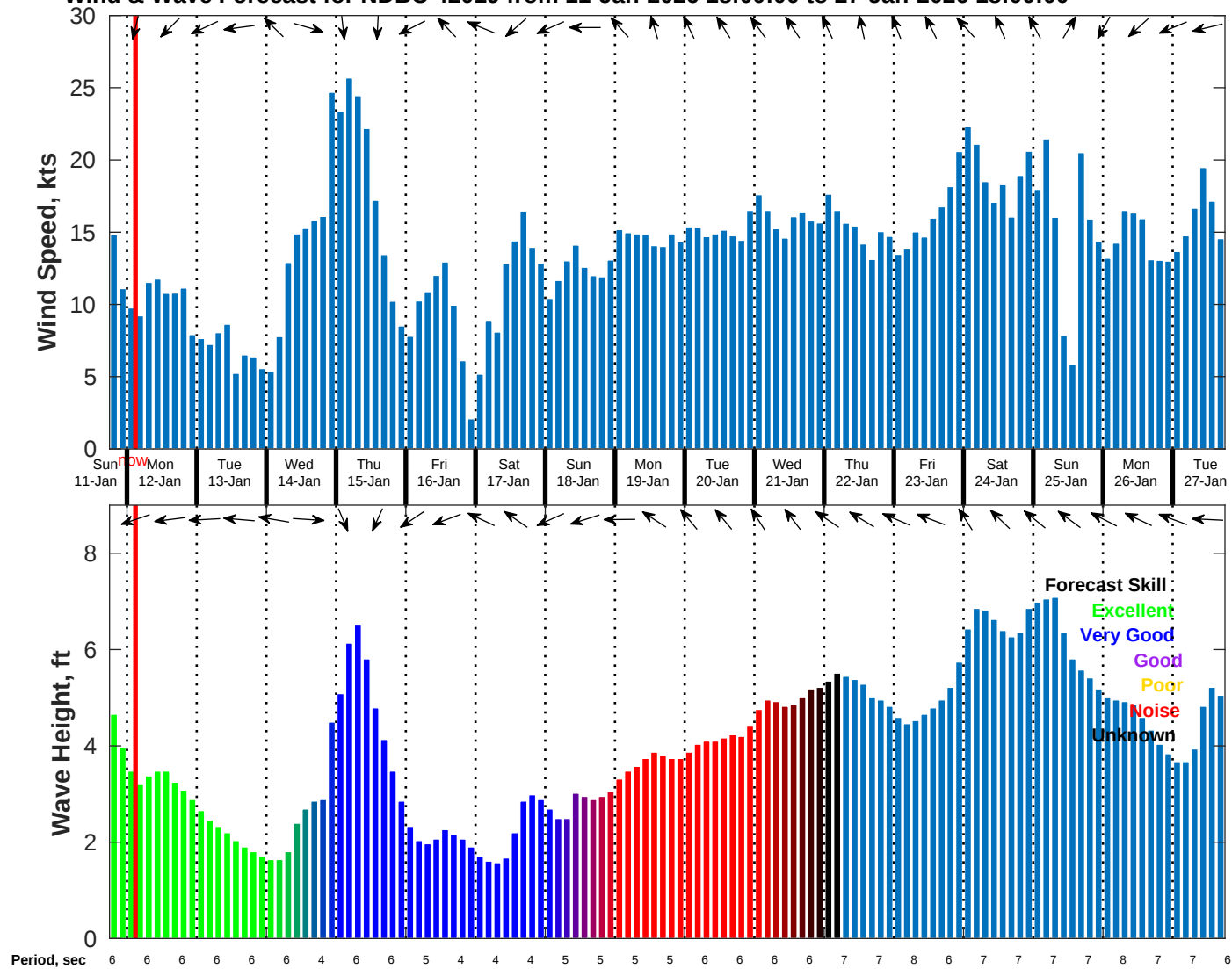
Wind & Wave Forecast for NDBC 42019 from 11-Jan-2026 18:00:00 to 27-Jan-2026 18:00:00
