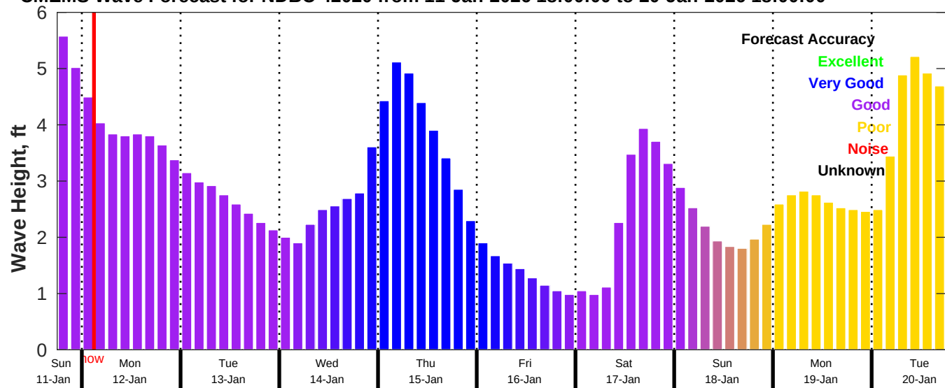
CMEMS Wave Forecast for NDBC 42020 from 11-Jan-2026 18:00:00 to 20-Jan-2026 18:00:00
