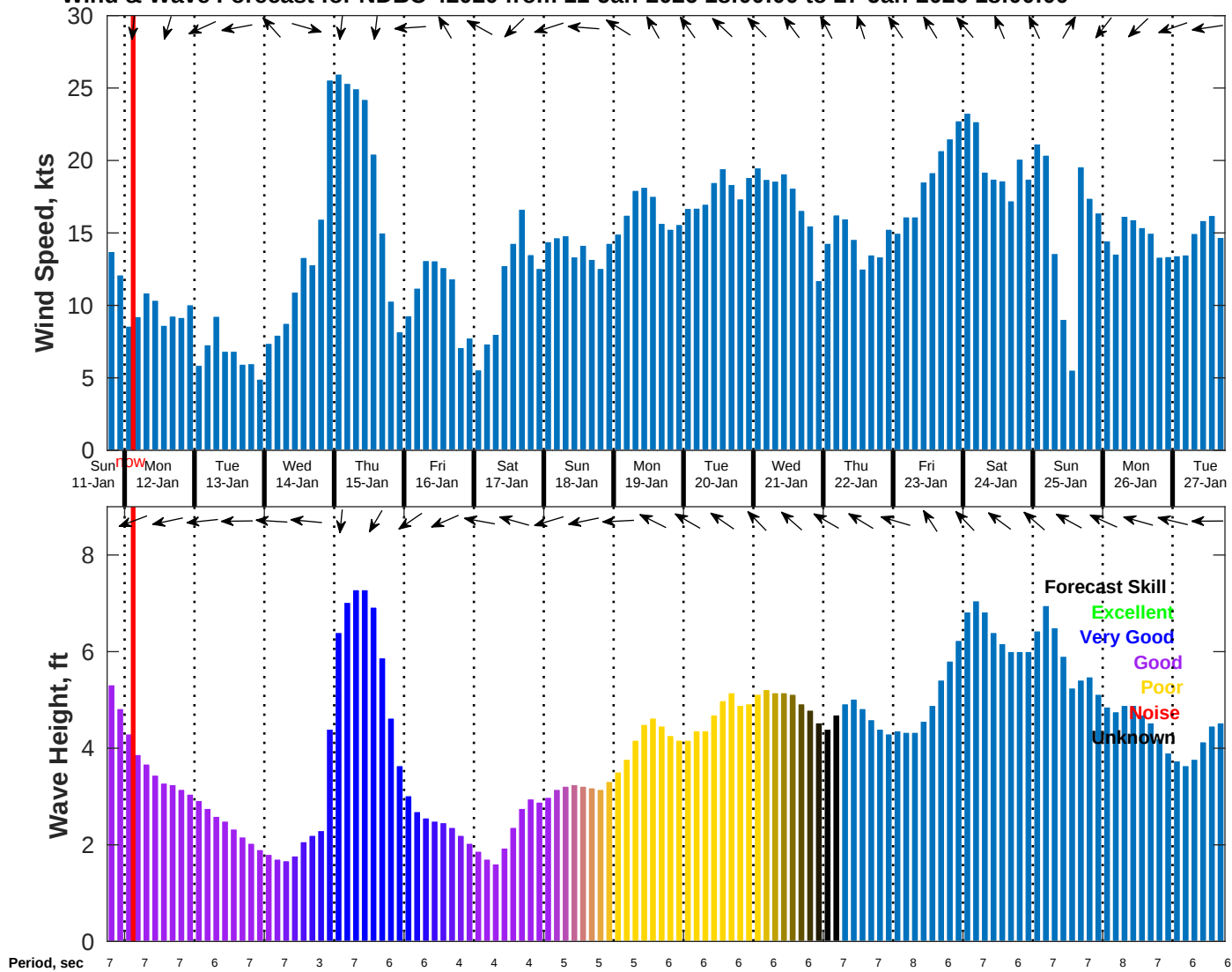
Wind & Wave Forecast for NDBC 42020 from 11-Jan-2026 18:00:00 to 27-Jan-2026 18:00:00
