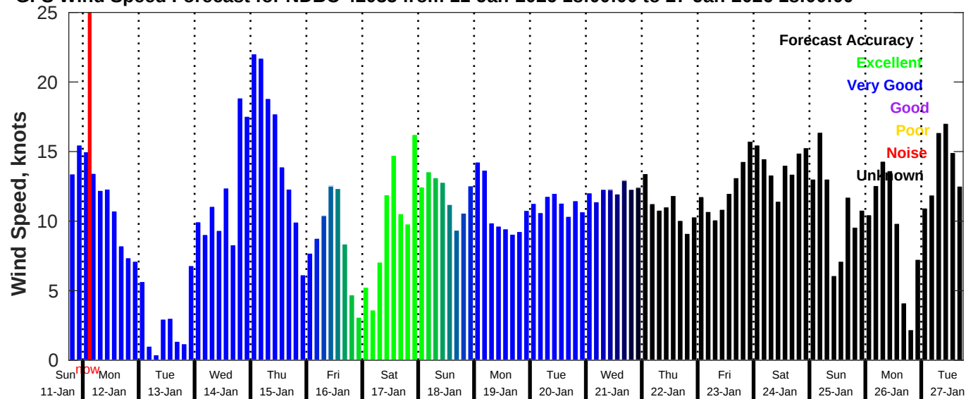
GFS Wind Speed Forecast for NDBC 42035 from 11-Jan-2026 18:00:00 to 27-Jan-2026 18:00:00
