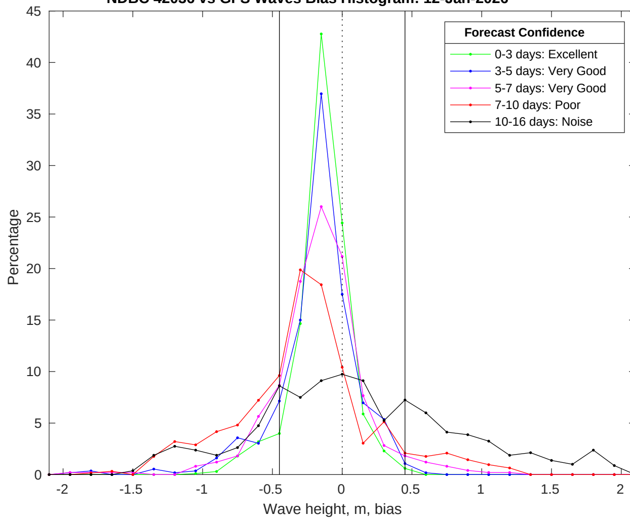
NDBC 42036 vs GFS Waves Bias Histogram: 12-Jan-2026
