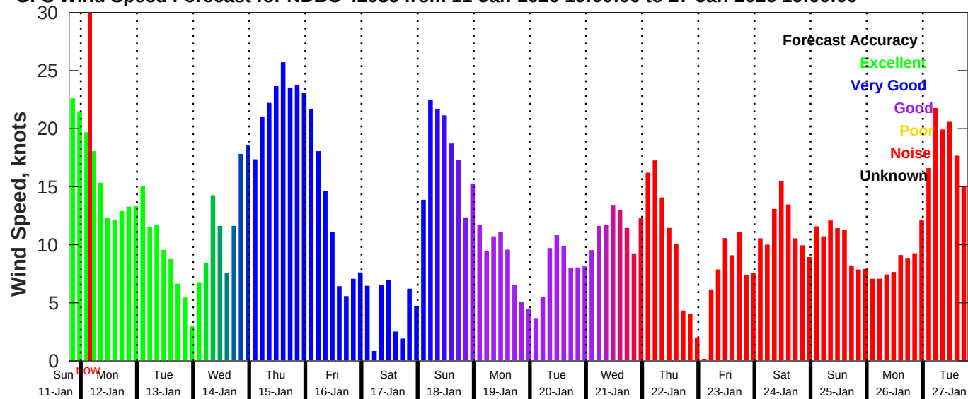
GFS Wind Speed Forecast for NDBC 42036 from 11-Jan-2026 19:00:00 to 27-Jan-2026 19:00:00
