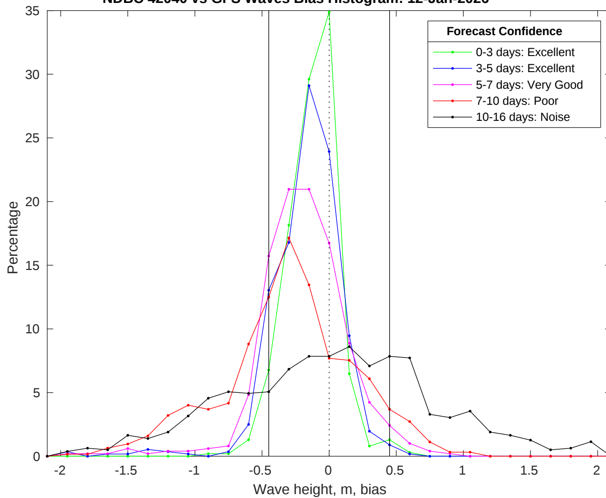
NDBC 42040 vs GFS Waves Bias Histogram: 12-Jan-2026
