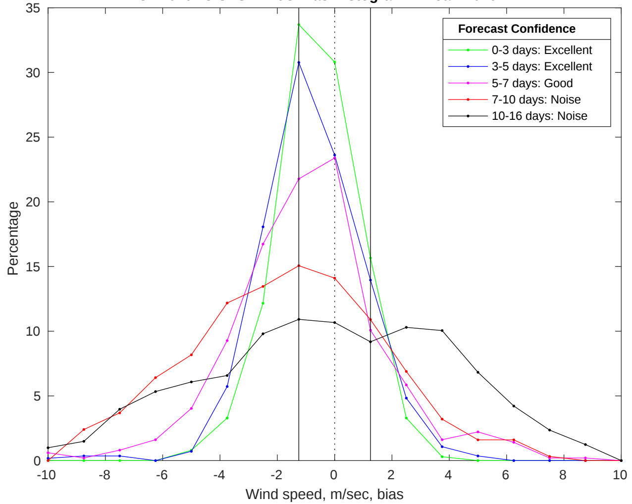
NDBC 42040 vs GFS Winds Bias Histogram: 12-Jan-2026
