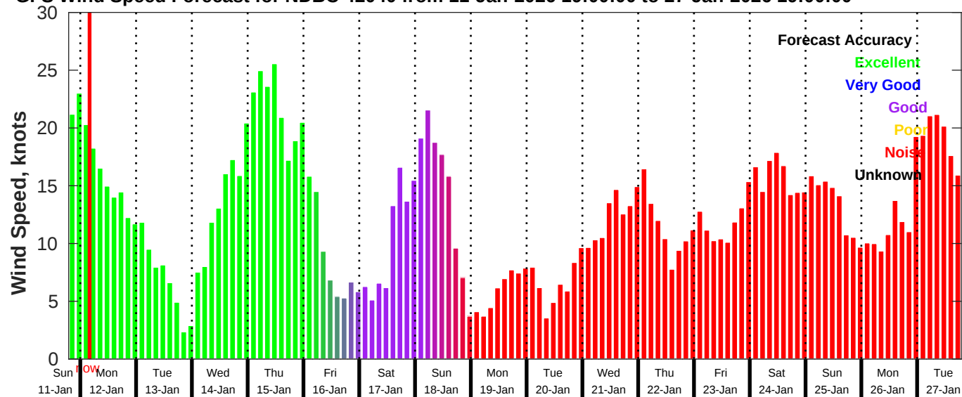
GFS Wind Speed Forecast for NDBC 42040 from 11-Jan-2026 19:00:00 to 27-Jan-2026 19:00:00
