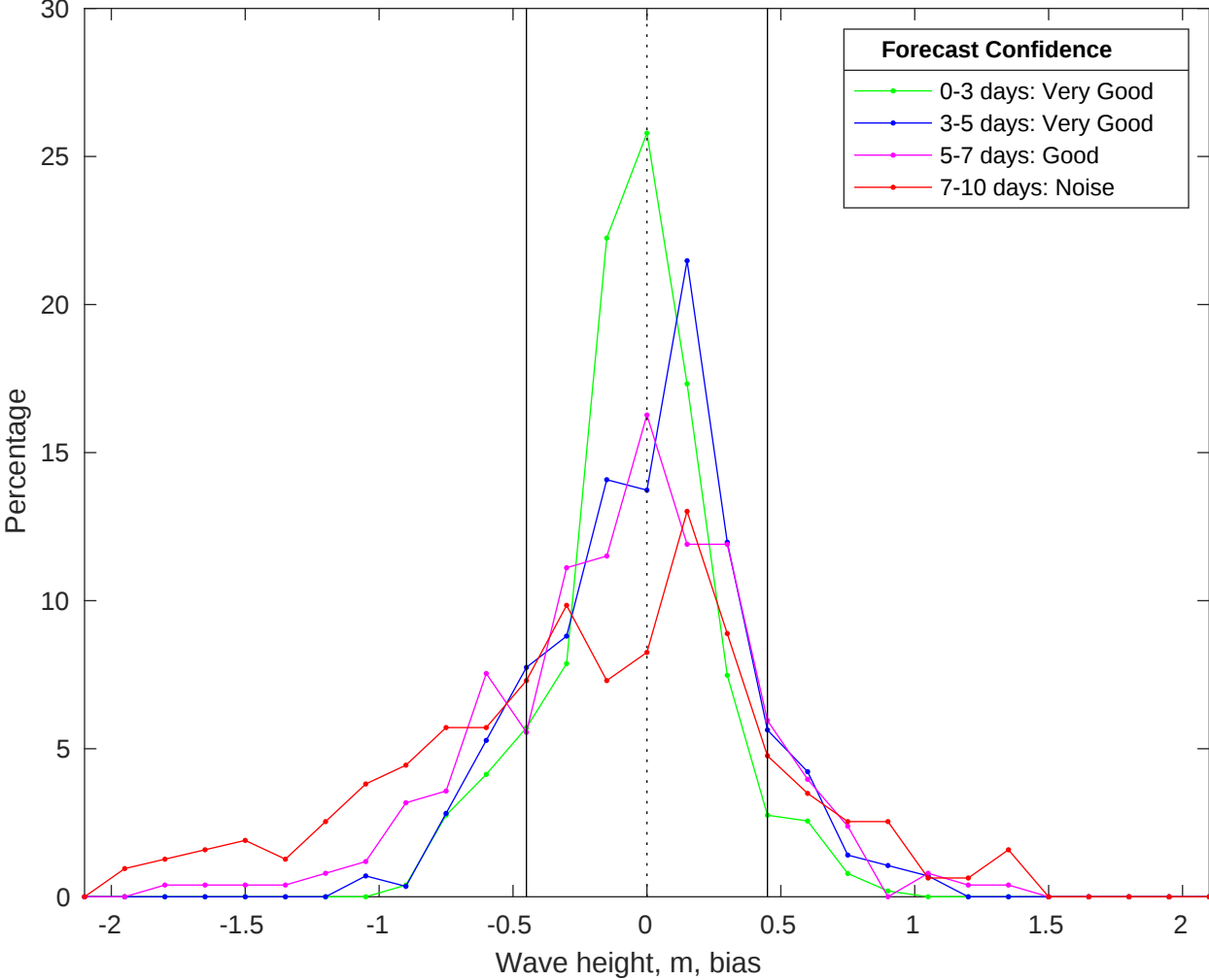
NDBC 46011 vs CMEMS Waves Bias Histogram: 12-Jan-2026
