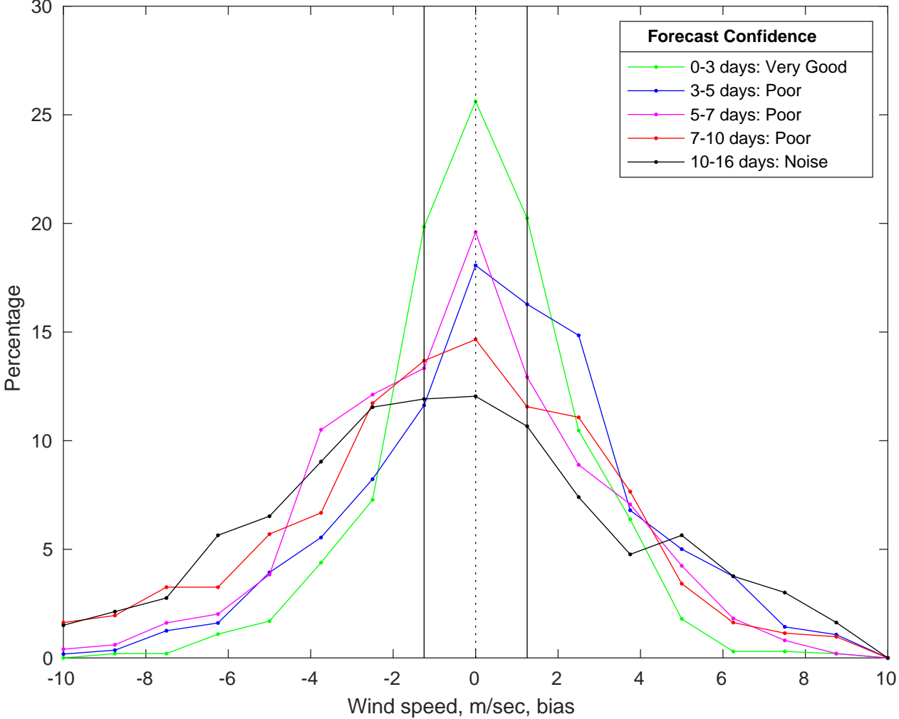
NDBC 46011 vs GFS Winds Bias Histogram: 12-Jan-2026
