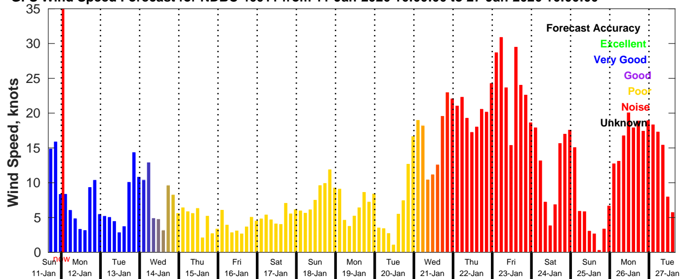
GFS Wind Speed Forecast for NDBC 46011 from 11-Jan-2026 16:00:00 to 27-Jan-2026 16:00:00
