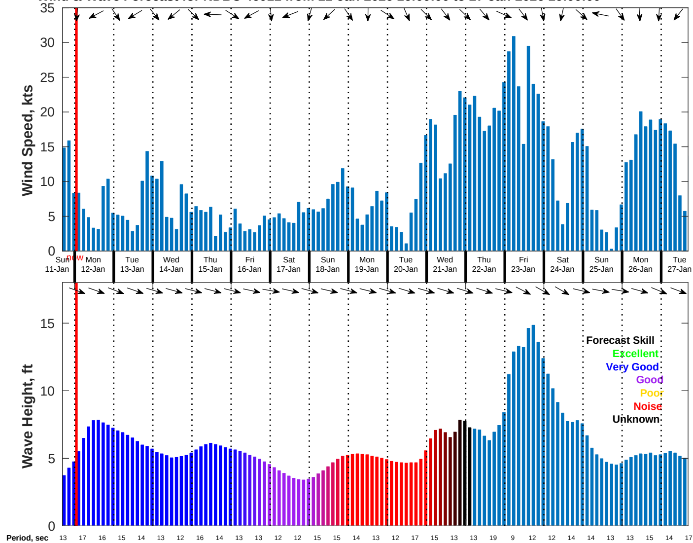
Wind & Wave Forecast for NDBC 46011 from 11-Jan-2026 16:00:00 to 27-Jan-2026 16:00:00
