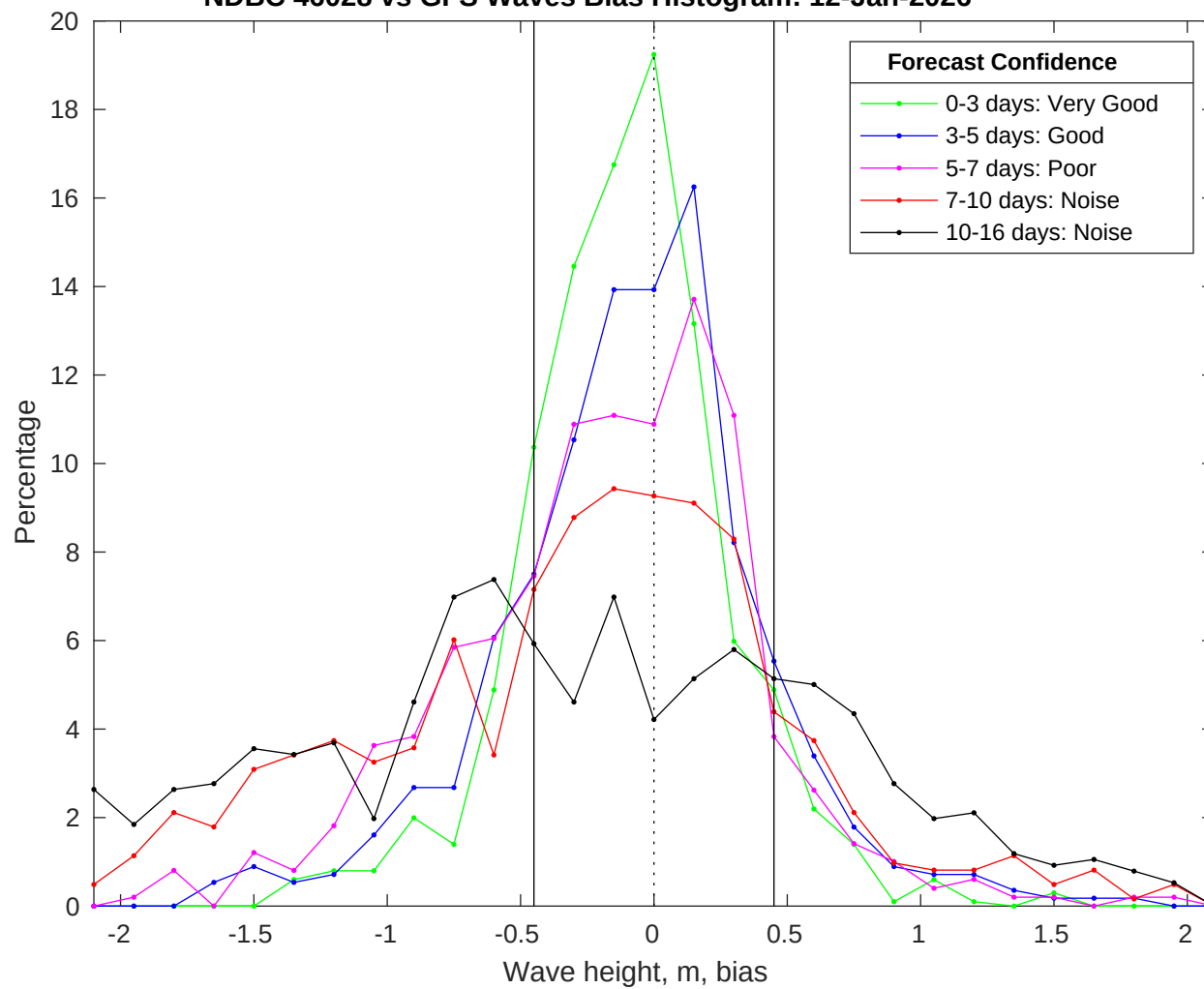
NDBC 46028 vs GFS Waves Bias Histogram: 12-Jan-2026
