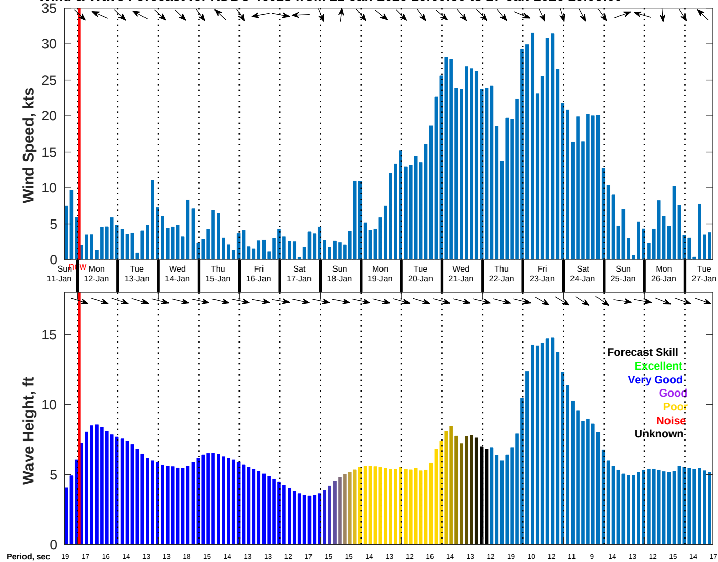
Wind & Wave Forecast for NDBC 46028 from 11-Jan-2026 16:00:00 to 27-Jan-2026 16:00:00
