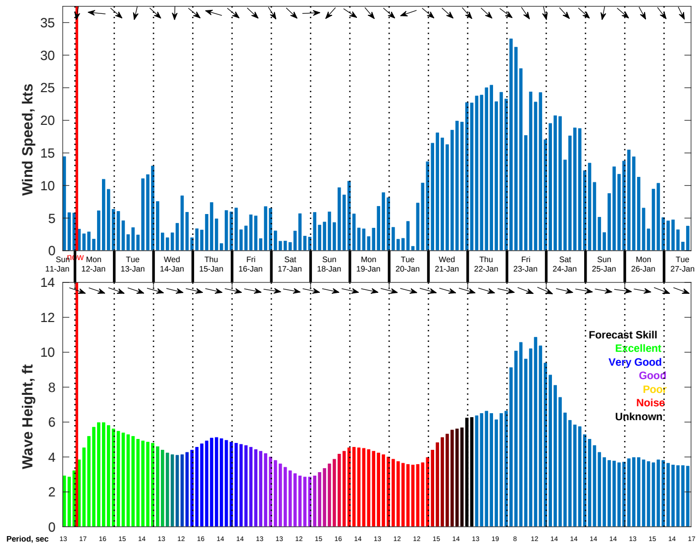
Wind & Wave Forecast for NDBC 46054 from 11-Jan-2026 16:00:00 to 27-Jan-2026 16:00:00
