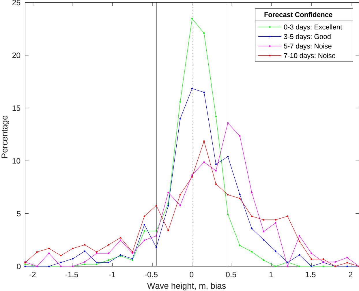
NDBC 46059 vs CMEMS Waves Bias Histogram: 12-Jan-2026
