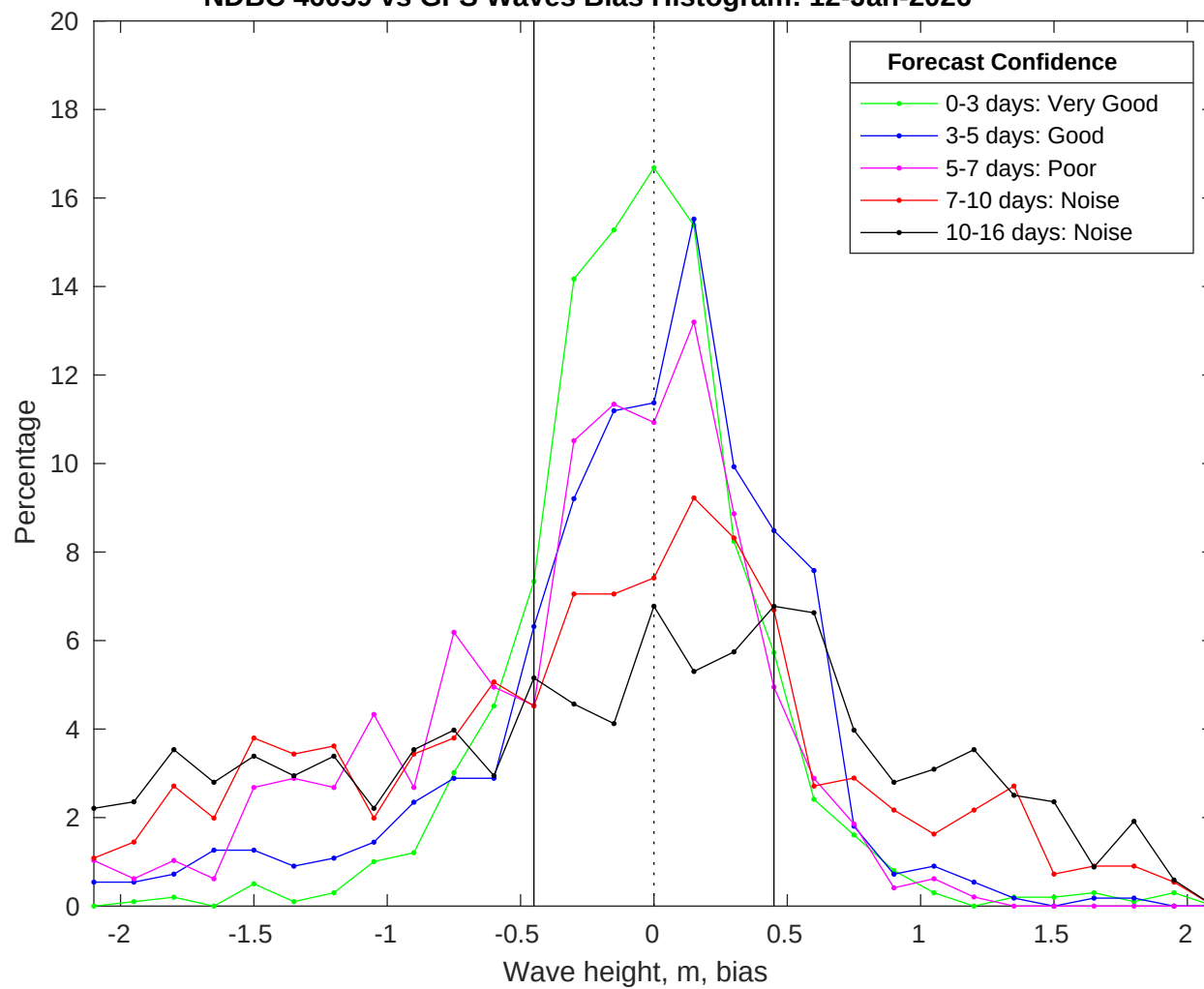
NDBC 46059 vs GFS Waves Bias Histogram: 12-Jan-2026
