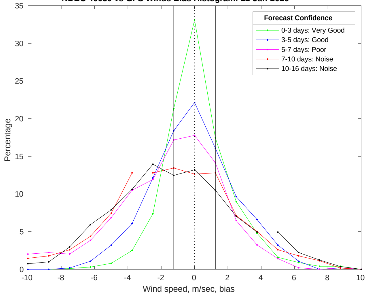
NDBC 46059 vs GFS Winds Bias Histogram: 12-Jan-2026
